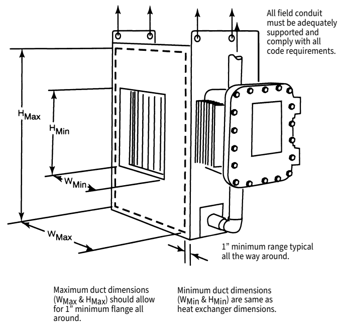
Figure 78. ULTRA-SAFE™ Mounting Configuration
